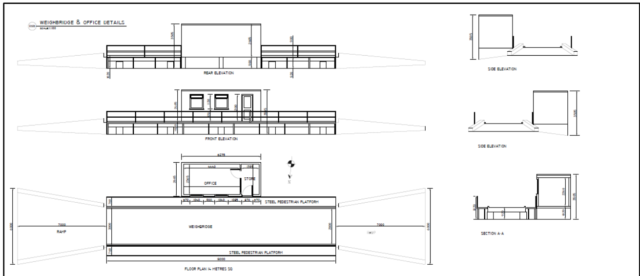
Figure 6.1 Prefabricated office and weighbridge (Source: Hydro Environmental Services Figure 108-1)
